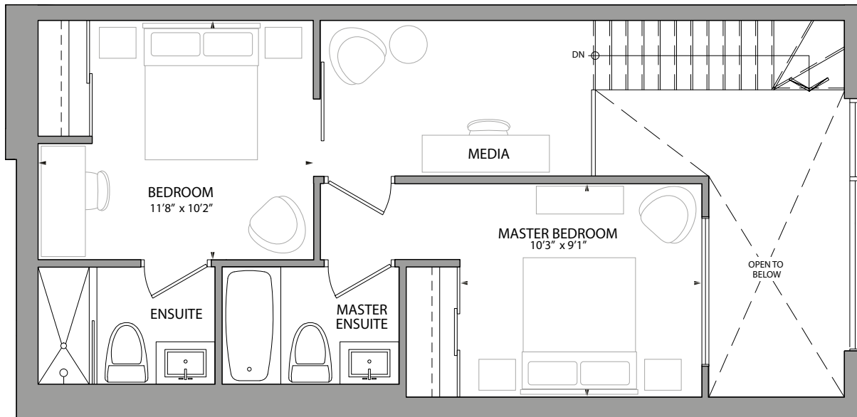
SECOND LEVEL
